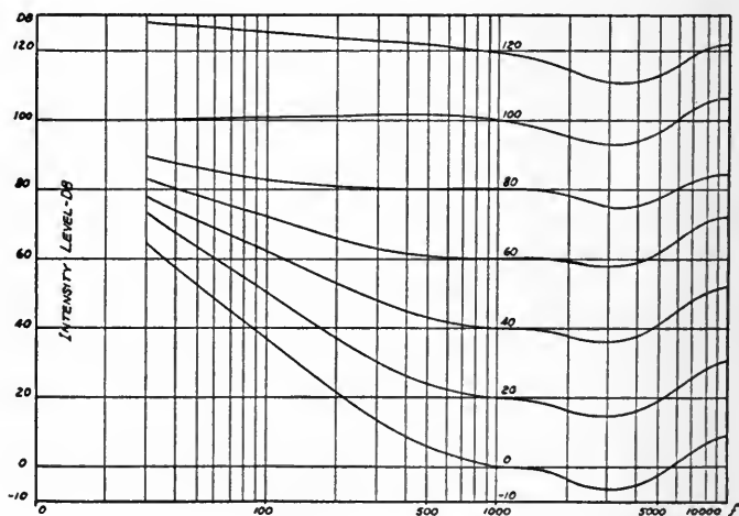
FIG. 1. Ear-sensitivity curves.
